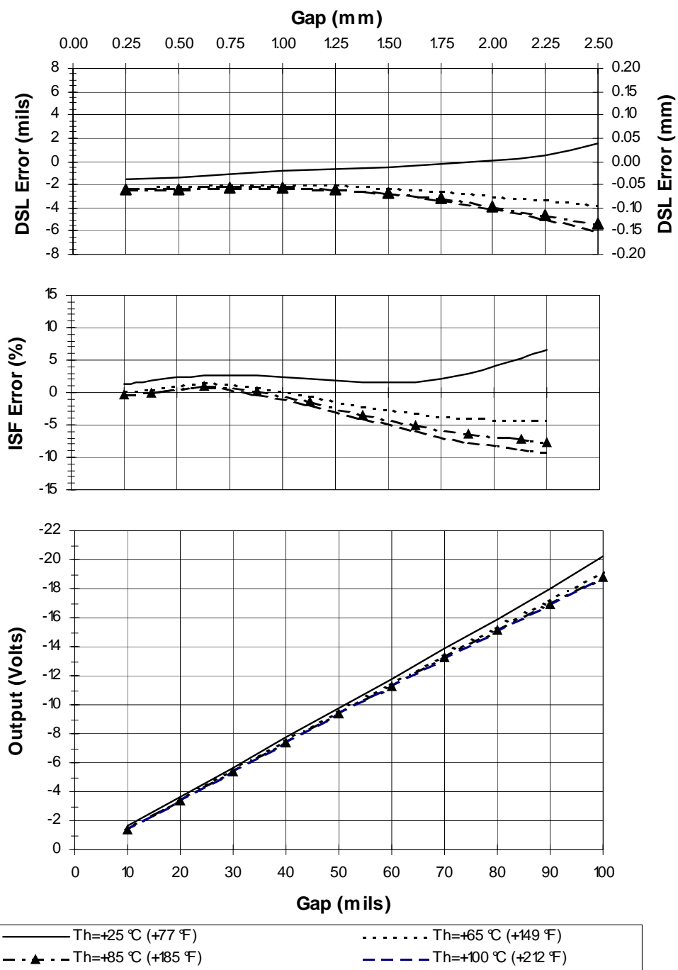
Figure 7 Typical 3300 XL 8 mm 9 m Proximitor® Sensor with 8 m of Extension Cable @ Th (Probe is at 25 °C)
