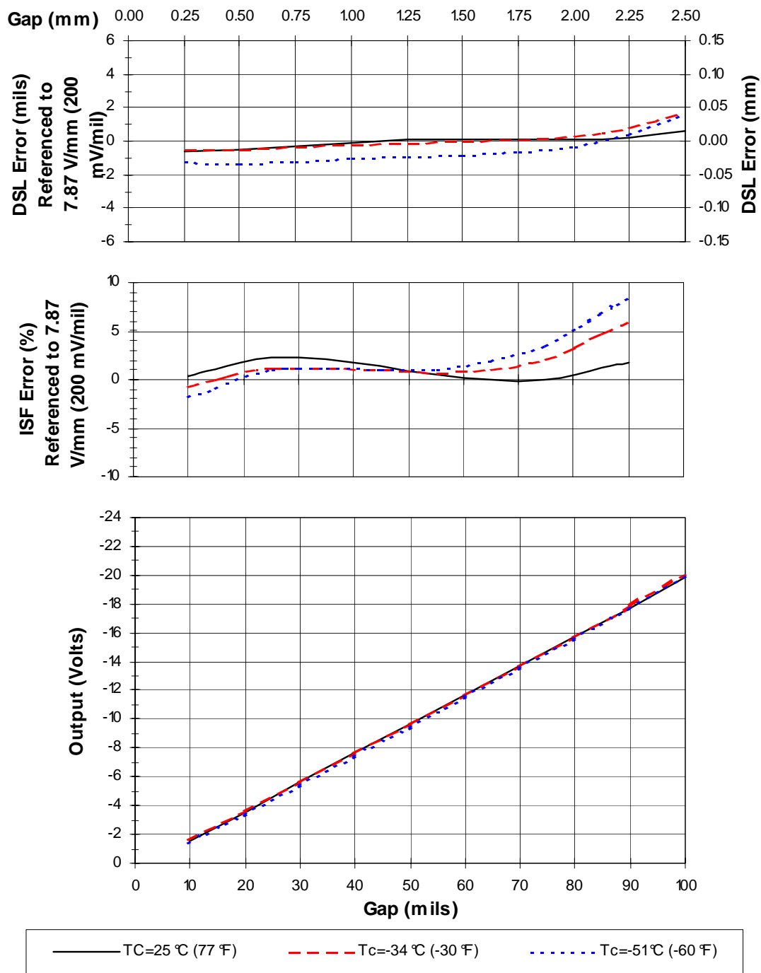
Figure 4 Typical 3300 XL 8 mm 5 m Proximitytor® Sensor with 4 m of Extension Cable @ T_c (Probe is at 25^\circ\text{C} )
